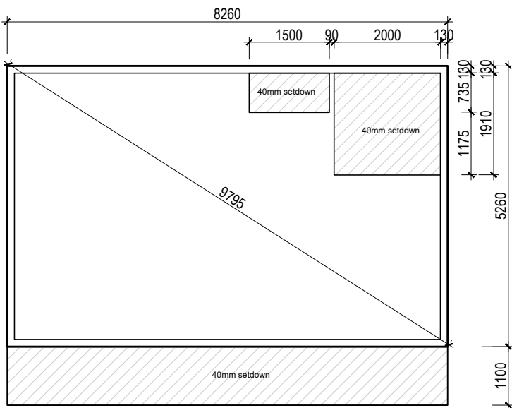
Slab Layout Plan
