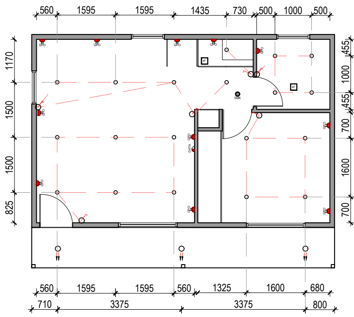
Electrical Layout Plan
