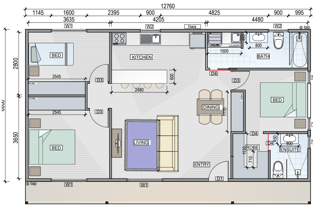
Ground Plan
