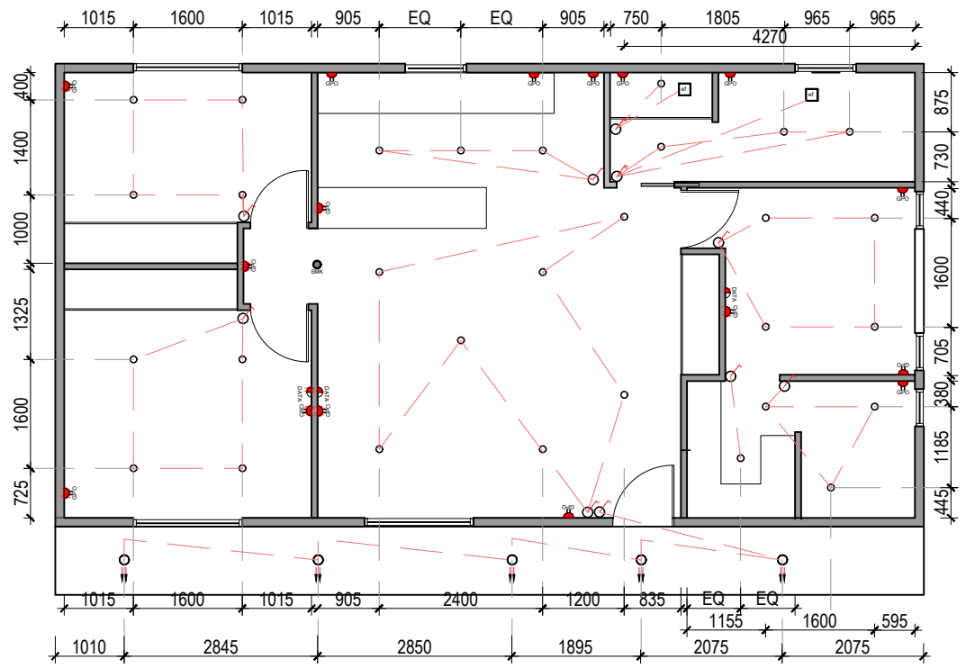
Electrical Layout Plan
