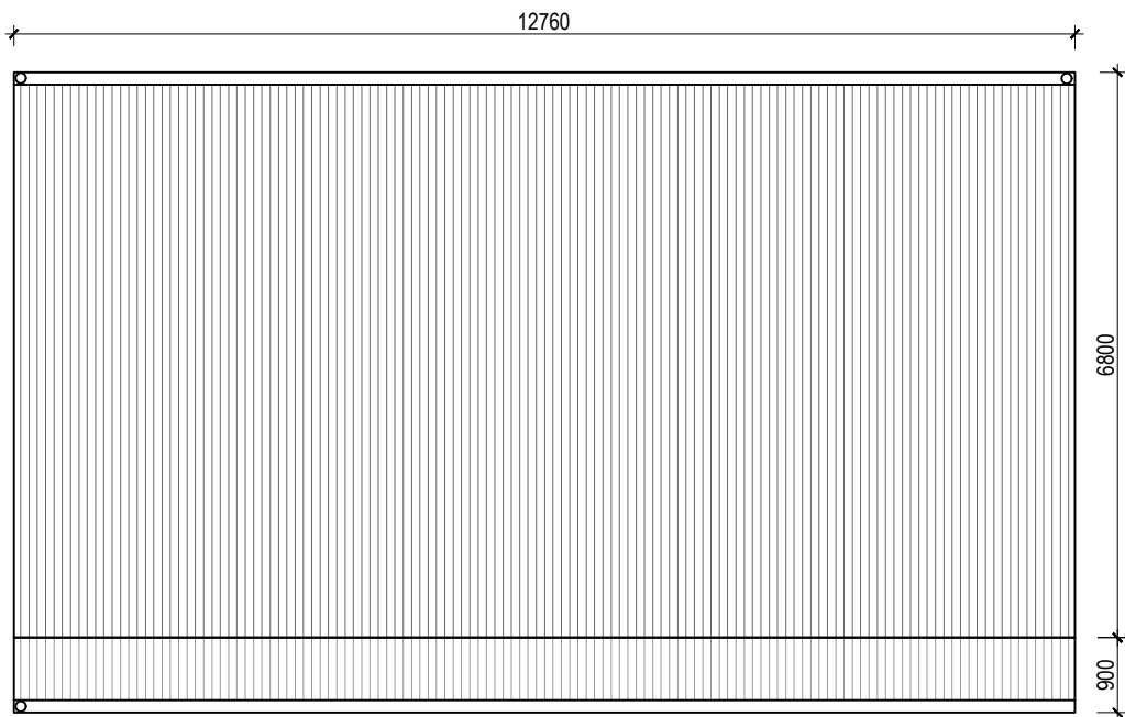
Roof Plan
