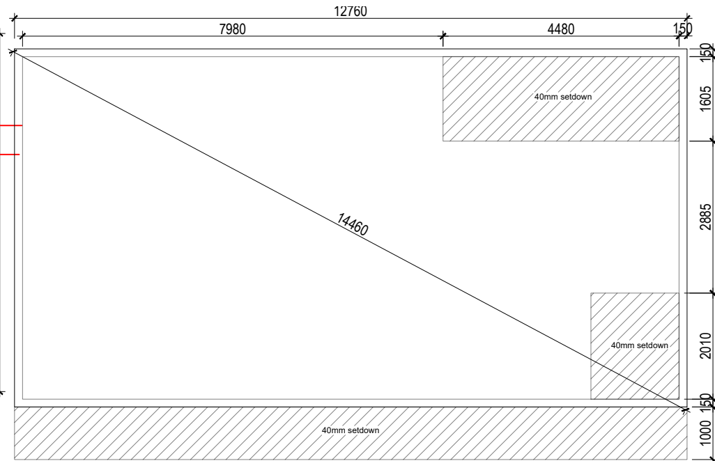
Slab Layout Plan
