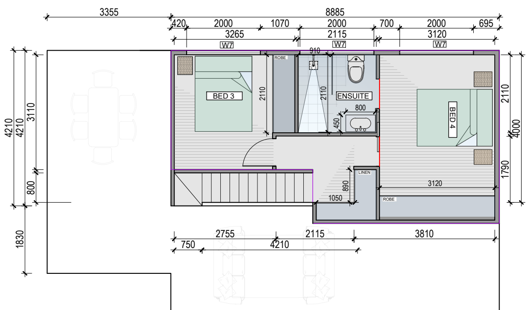
Mezzanine Plan
