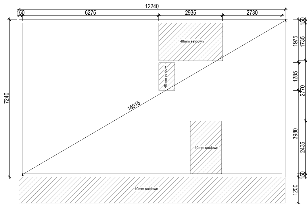
Slab Layout Plan
