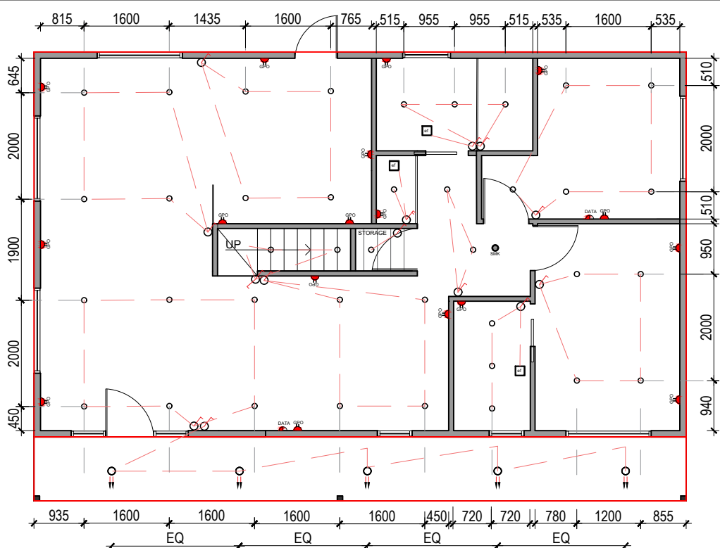
Electrical Layout Plan
