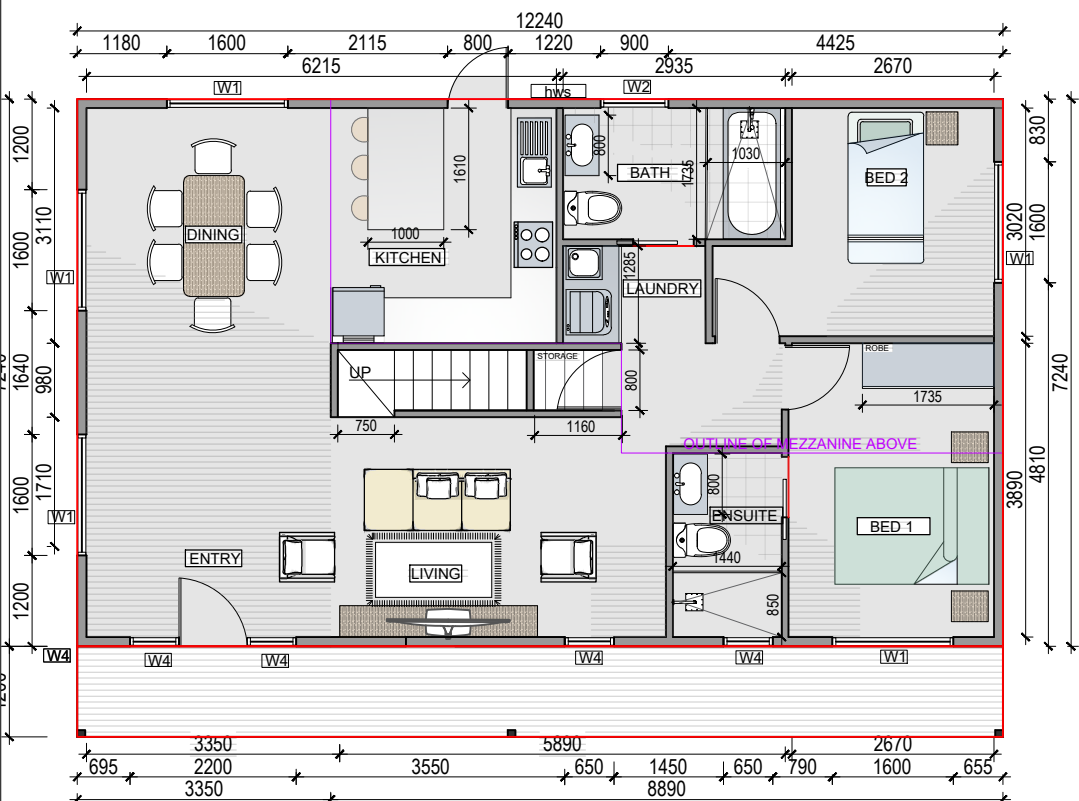
Ground Plan
