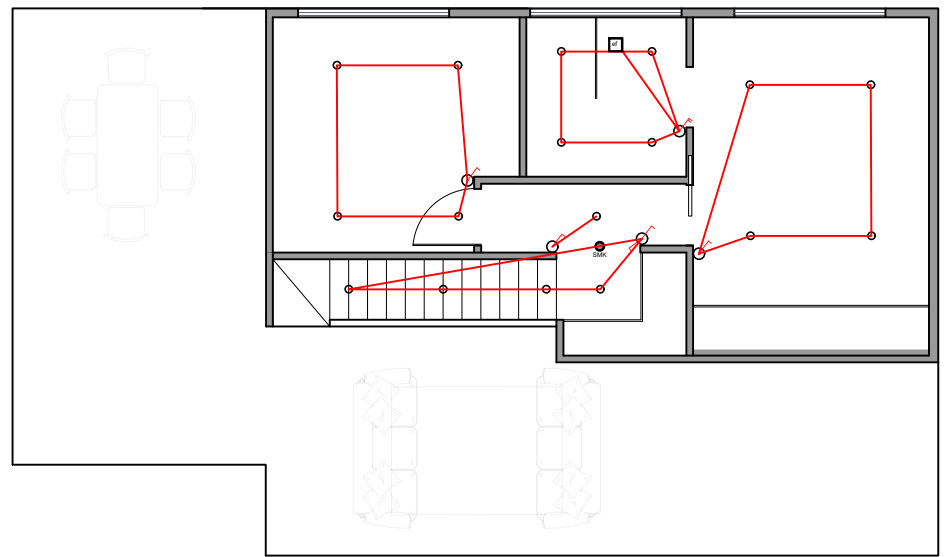
Mezzanine Plan
